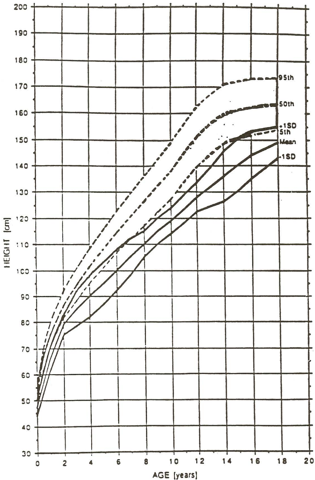
Figure 51 Growth curve for height in females with Noonan syndrome (solid lines) compared to normal values (dashed lines). Data obtained in 48 Noonan syndrome females from a collaborative retrospective review. (From Witt DR, et al. Clin Genet 1986; 30:150.)
